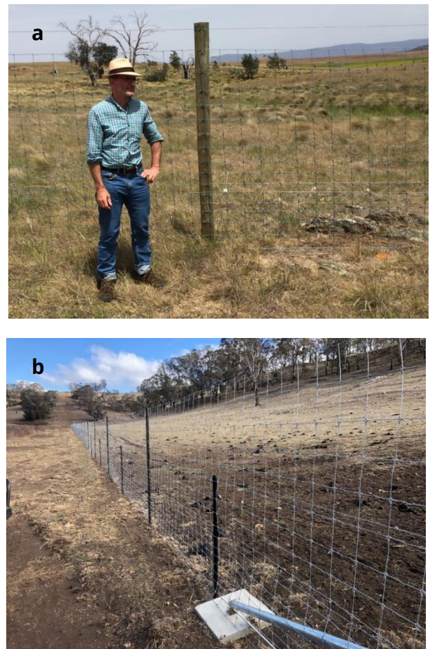
Figure 2. Two deer fence designs, both \geq 190 cm in height. (a) This design uses 190-cm-high netting with one high-tensile wire 15 cm above that and treated timber posts spaced at 5 m. (b) This design uses 190 cm-high netting (17/190/15) with steel star posts spaced at 5 m intervals (note alternating taller and shorter star posts).
